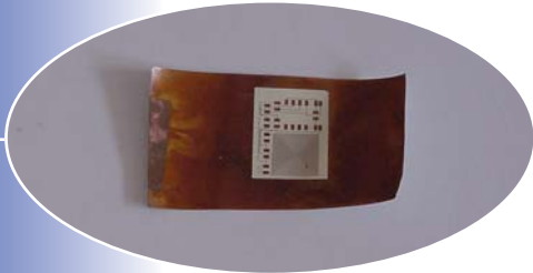
Micro Heater Fabricated from Copper Plated LCP. (Dimensions 16 mm x 13 mm).
